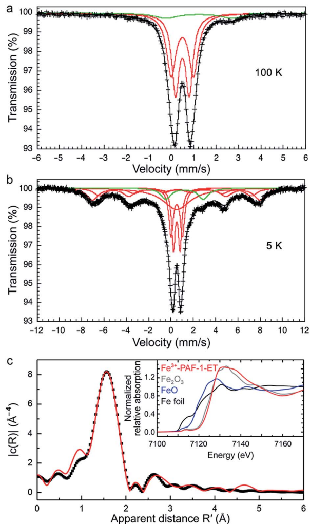
Fig. 4 Iron-57 Mössbauer spectra of PAF-1-ET obtained at (a) 100 and (b) 5 K. Red and green fits were assigned to iron(III) (91%) and iron(II) (9%), respectively. The total fit is shown in black. (c) The Fourier transform of the k^3 -weighted iron K-edge EXAFS data of iron(III) adsorbed in PAF-1-ET (black dots); the best two-shell fit (red curve) was achieved with an immediate coordination environment of six O atoms at a distance of 2.00(1) Å and 12 C atoms at a distance of 3.06(4) Å; (inset) room-temperature XANES spectra obtained at the iron K-edge for PAF-1-ET (red curve) and \text{Fe}_2\text{O}_3 , FeO, and Fe foil (gray, blue, and black curves, respectively).
