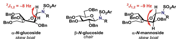
Fig. 1 Observed conformations of N -glycosides determined from 1 H-NMR coupling constants.
