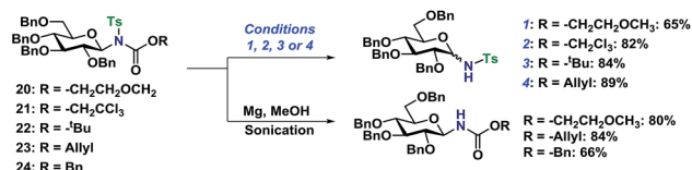
Scheme 6 Orthogonal deprotection of tosyl-protected N -glycosides. Reaction conditions: (1) \text{K}_2\text{CO}_3 (2 equiv.), 0.02 M in MeOH, reflux, 4 h. (2) Zn (8 equiv.), 0.12 M in AcOH, 70 °C, 2 h. (3) TFA (20 equiv.), 0.03 M in \text{CH}_2\text{Cl}_2 , rt, 8 h. (4) \text{PhSiH}_3 (4 equiv.), \text{Pd}(\text{PPh}_3)_4 (0.05 equiv.), 0.75 M in \text{CH}_2\text{Cl}_2 , rt, overnight.
