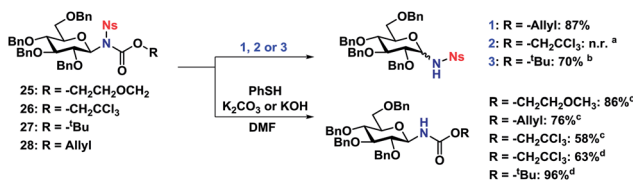
Scheme 7 Orthogonal deprotection of nosyl-protected N -glycosides. Reaction conditions (1) sodium p -toluenesulfonate (1.1 equiv.), \text{Pd}(\text{PPh}_3)_4 (0.1 equiv.), 0.012 M in MeOH/THF 1 : 2, rt, 1.5 h. (2) Zn (20 equiv.), 0.025 M in AcOH, rt, 0.5 h. (3) TFA (20 equiv.), 0.4 M in \text{CH}_2\text{Cl}_2 , rt, o.n. a Resulted in reduction of the Ns nitro group to the corresponding amine. b Glycosylation and deprotection carried out in a single step, 70% overall yield. c \text{K}_2\text{CO}_3 used as base. d KOH used as base.
