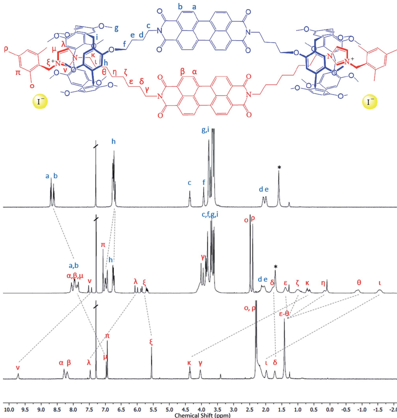
Fig. 2 1 H NMR spectra illustrating formation of the handcuff structure, 4. Top: bis-pillararene component, 1; middle: handcuff 4; bottom – non-interlocked bis-imidazolium rod, 6. See Fig. S25† for 1 H NMR spectra of handcuff 5.
