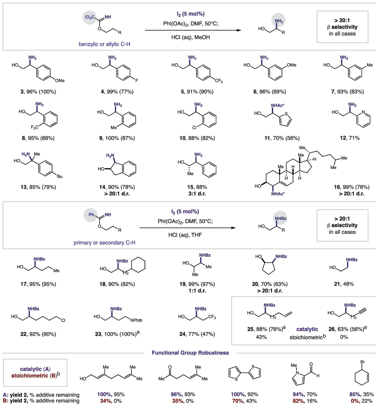
Fig. 3 Synthetic utility of iodine-catalyzed β C-H amination of imidates. Conditions: 0.4 mmol imidate, I_2 (5 mol%), PhI(OAc)_2 (1.2 equiv.), DMF (0.2 M), 50 °C. 1 H NMR yield of oxazoline determined vs. standard. Hydrolysis with HCl (2 M) affords amino alcohol (isolated yield, in parenthesis). a Isolated yield of oxazoline. b Stoichiometric NaI (ref. 12). Ac* refers to trichloroacetamide. Functional group robustness: C-H amination yield, % additive remaining.
