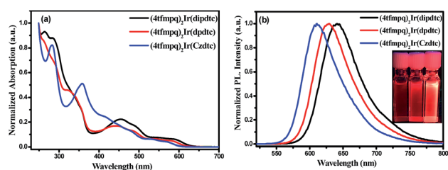
Fig. 3 The UV-vis absorption (a) and emission (b) spectra of the three complexes (4tfmpq)_2Ir(dipdte) , (4tfmpq)_2Ir(dpdtc) and (4tfmpq)_2Ir(Czdtc) in degassed dichloromethane ( 5 \times 10^{-5} M) at room temperature.
