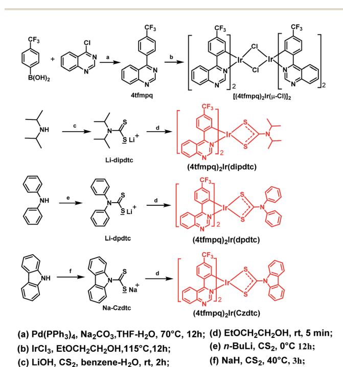
Scheme 1 The synthetic routes to the ligands and complexes.
