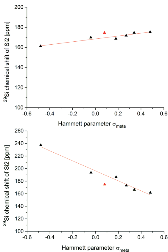
Fig. 4 Plots of the Hammett parameters \sigma_{\text{m}} vs. ^{29}\text{Si} chemical shifts of the privo silicon vertices of ligato ( 5a–f ; top) and privo functionalized hexasilabenzpolarenes ( 6a–f ; bottom). The data pair marked with red triangles corresponds to the unfunctionalized hexaaryl derivative 2 .
