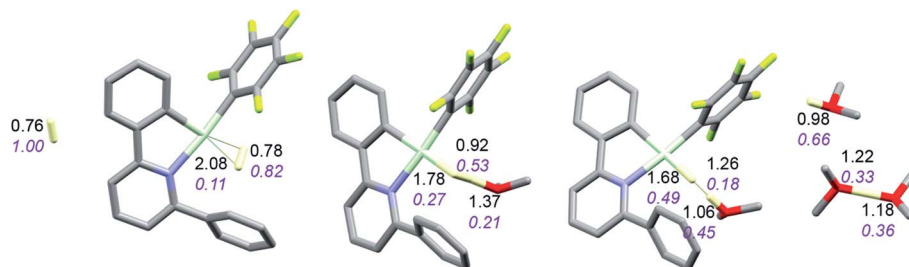
Fig. 9 Activation of \text{H}_2 by \text{LAu}^+/\text{OMe}_2 . Bond lengths in Å, Wiberg bond indexes shown in purple and italics.
