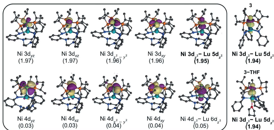
Fig. 5 CASSCF-derived natural orbitals for 4 , shown with occupation numbers. Similar natural orbitals were observed for 3 and 3 -THF. Shown to the right, the Ni 3d z 2 natural orbitals for 3 and 3 -THF, where a minor contribution from Lu 5d z 2 is visible.
