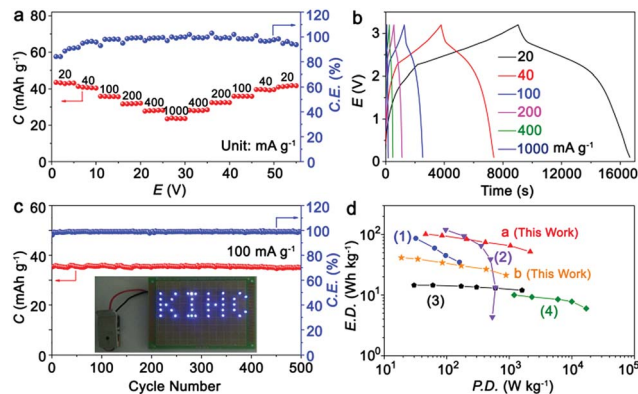
Fig. 5 (a) Rate capability; (b) charge/discharge curves at different rates; (c) cycling performance of the KIHIC at 100 \text{ mA g}^{-1} for 500 cycles; and (d) Ragone plots of the KIHIC of K_2TP//AC , and other reported KIHICs, a KIB, and an EDLC. (1) Soft carbon// K_{0.7}Fe_{0.5}Mn_{0.5}O_2 (KIB), ref. 12; (2) soft carbon//AC (KIHIC), ref. 6; (3) graphite//AC (KIHIC), ref. 5; (4) AC//AC (EDLC), ref. 35. The current density, capacity, power density and energy density are all based on the total mass of active materials in both electrodes. Exceptionally, plot b is based on the mass of both electrodes and the electrolyte.
