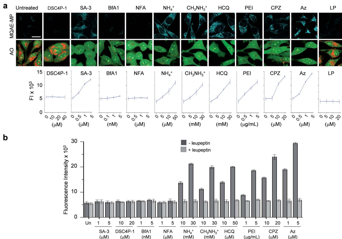
Fig. 5 Detection of lysosomal chloride ions in cells treated with various substances using MQAE-MP. (a) HeLa cells were incubated for 6 h with each substance (concentration: 40 \mu M DSC4P-1, 5 \mu M SA-3, 5 nM BfA1, 5 \mu M NFA, 30 mM NH 4 + , 30 mM CH 3 NH 3 + , 50 \mu M HCQ, 5 \mu g mL -1 PEI, 20 \mu M CPZ, 5 \mu M Az and 50 \mu M LP) and then treated for 30 min with 5 mM MQAE-MP or 100 nM acridine orange (AO). Cell images were obtained by using confocal fluorescence microscopy (scale bar: 10 \mu m). Graph shows the fluorescence intensities (FI) of cells treated with indicated concentrations of each substance for 6 h (see Fig. S10† for complete images). Fluorescence intensities of MQAE-MP in the cells were analyzed by using ZEN software. (b) HeLa cells were treated with each substance for 6 h. Cathepsin B activity of the isolated cytosolic fraction was measured by using a fluorogenic substrate MR-(RR) 2 in the absence and presence of leupeptin (mean \pm s.d., n = 3).
