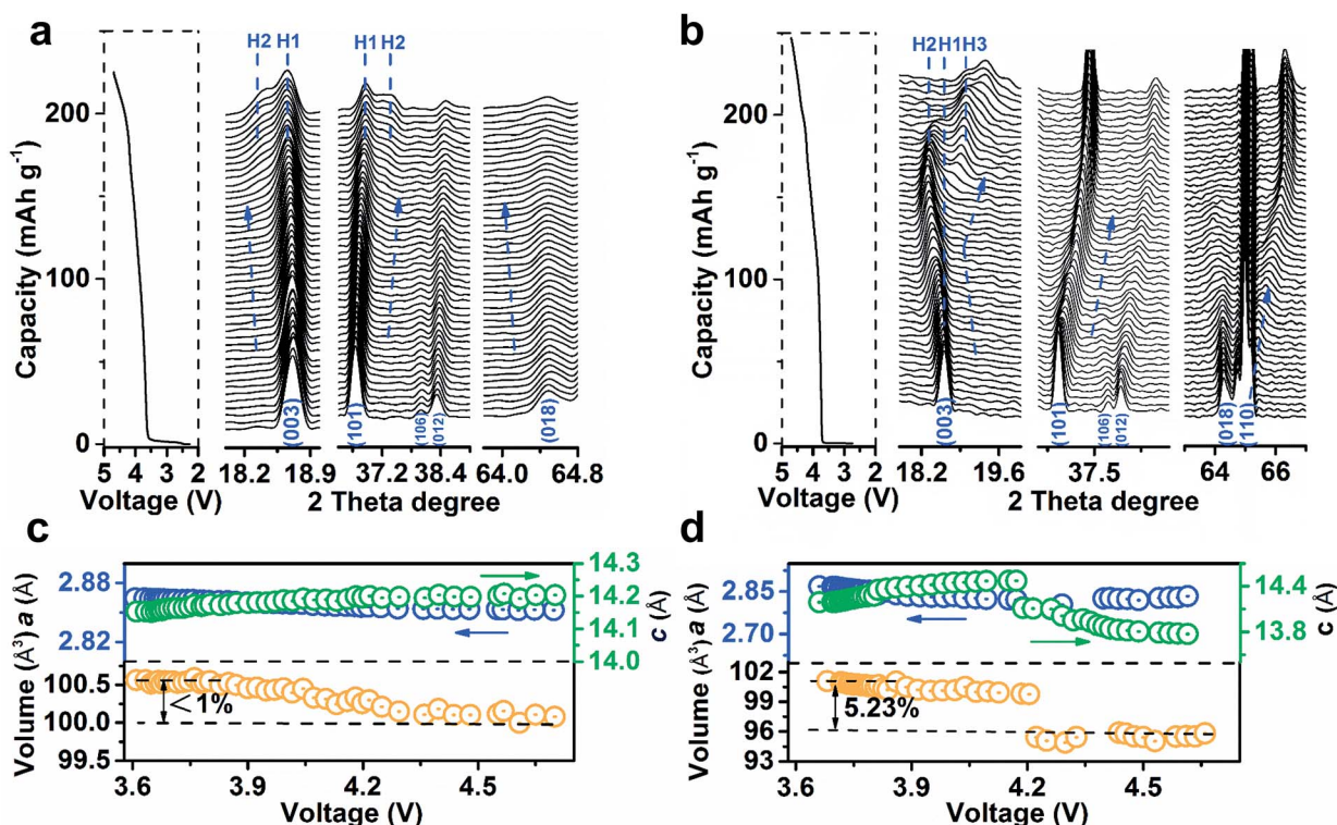
Fig. 4 Structural evolution of LiNi 0.9 Co 0.07 Mg 0.03 O 2 (a and c) and NCM811 (b and d). (a and b) In situ XRD patterns at selected 2 \theta regions and the corresponding galvanostatic curves on first charging. (c and d) The variation of lattice parameters and cell volumes as a function of voltage.
