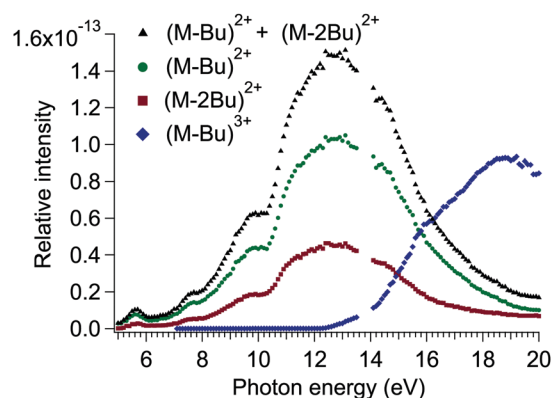
Fig. 6 Action spectra of (M-Bu) 2+ , (M-2Bu) 2+ and (M-Bu) 3+ formation from the precursor ion M^{2+} , between 5 and 20 eV.
