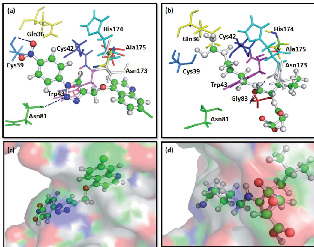
Fig. 3 Docking interactions of T7 and E64 , a known standard FP2 inhibitor with FP2: PDB ID 3BPF; (a) binding interaction of compound T7 with FP2 showing \pi - \pi stacking between Trp43 and aromatic triazole ring (represented with red coloured dashes) and two H-bonds between the ligand and Cys39 and Asn81 of FP2 (represented with dark blue coloured dashes). (b) Showing H-bond interaction of E64 with the Gly83 and Asn173 of FP2 (represented with dark blue coloured dashes). (c) Surface view of T7 into the active site groove of the enzyme: (d) Surface pose of E64 with FP2.
