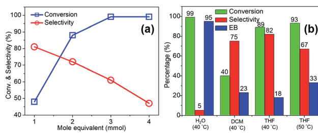
Fig. 7 (a) Variation in the conversion and selectivity of m -nitrostyrene at 45 °C with THDB mole equivalent in THF (b) conversion and selectivity of o -bromostyrene with 1.1 equivalent of THDB in different solvents. EB: ethylbenzene.
