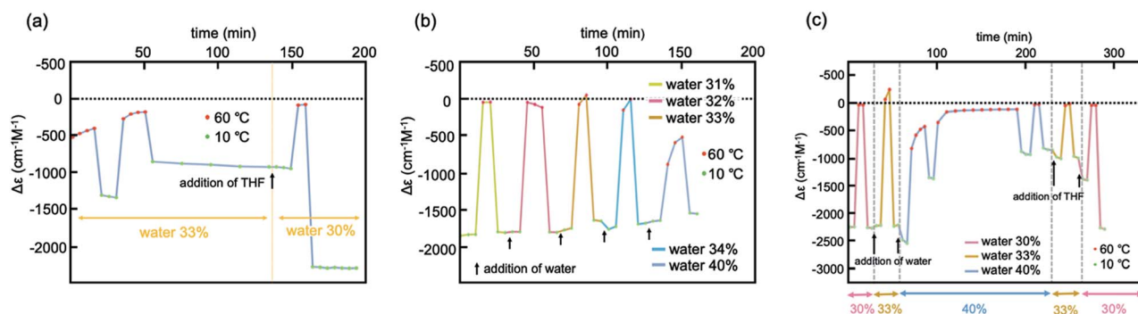
Fig. 5 Experiments using (M)-1/(P)-2 (1 : 1) with change in water content in water-THF (10 \mu M) at 371 nm. (a) From 33% to 30% by adding THF; (b) from 30% to 31, 32, 33, and 34% by adding water; (c) from 30% to 33%, and 40% by adding water, and then to 33% by adding THF.
