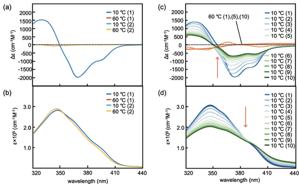
Fig. 2 (a) CD and (b) UV-vis spectra of (M)-1/(P)-2 (1 : 1) in 30% water-THF (10 \mu\text{M} ) at 60^\circ \text{C} and 10^\circ \text{C} . (c) CD and (d) UV-vis spectra of (M)-1/(P)-2 (1 : 1) in 33% water-THF (10 \mu\text{M} ) at 60^\circ \text{C} and 10^\circ \text{C} . The numbers of heating/cooling cycles is shown in parentheses. See Fig. S8a† for details of the spectra in (c) and (d).
