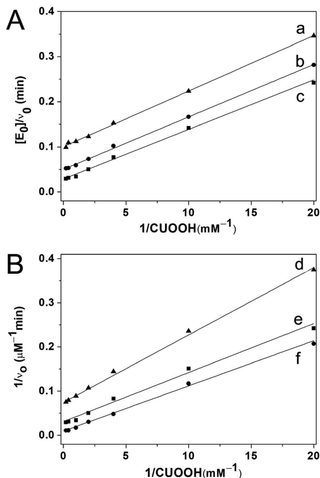
Fig. 8 (A) [E_0]/v_0 (min) vs. 1/[CUOOH] ( \text{mM}^{-1} ) for 1 μM PNTegel in PBS, pH 7.0 and 37 °C, at [TNB] = 0.04 mM (a), 0.10 mM (b), 0.15 mM (c). (B) Lineweaver-Burk plots obtained for the catalytic reaction in the presence of different concentration of PNTegel ( [PNTegel] = 0.5 μM (d), 1 μM (e), 2 μM (f)) at pH 7.0 and 37 °C. The initial CUOOH concentration was fixed to 0.25 mM.
