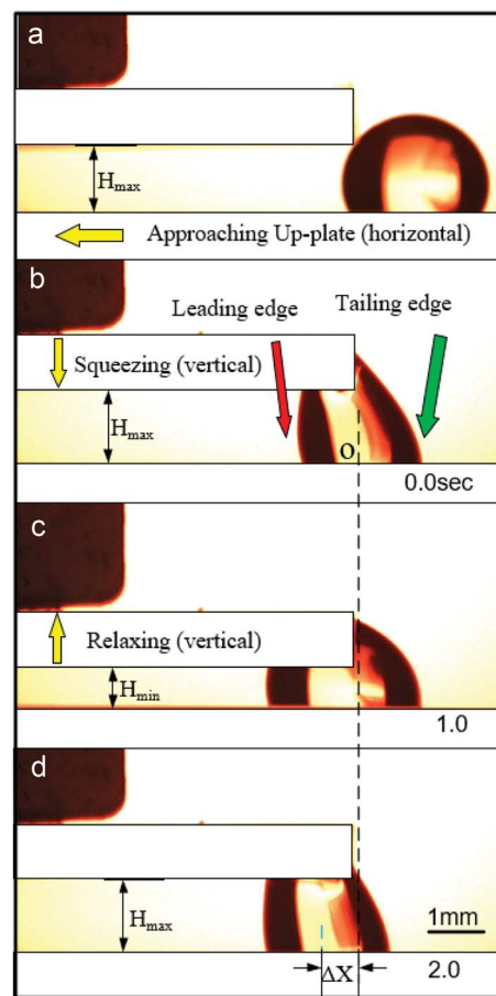
Fig. 1 (a) Initial position of the droplet before bridge formation. (b) Initial position of the liquid bridge after bridge formation. The gap width is represented by H_{max} . (c) The bridge is squeezed for \Delta H , and the gap width is represented by H_{min} . (d) Subsequently, the squeezed liquid bridge was relaxed for \Delta H to H_{max} to finish the ratchet-like cycle.
