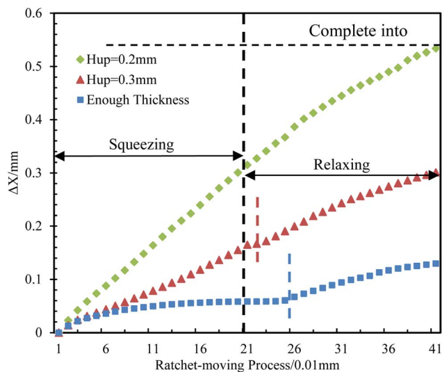
Fig. 8 Simulation of the value of \Delta X versus |\Delta H| for the same situation as shown in Fig. 3 but with three different values of H_{up} at 0.2 mm, 0.3 mm and no limit.
