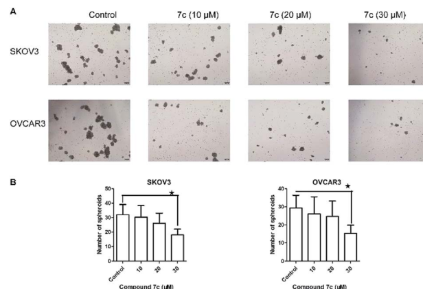
Fig. 6 (A) Compound 7c inhibited the sphere formation ability of SKOV3 and OVCAR3 cells. Single cells were seeded in ultra-low attachment plates. Then cells were seeded to form secondary generation incubated with compound 7c, and the spheroids were photographed. (B) Quantitative analysis of the spheroid numbers was shown. * P < 0.05 .
