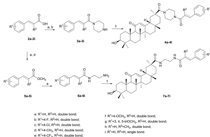
Scheme 1 Reagents and conditions: (a) SOCl 2 , r.t., 1 h; (b) piperazine, CH 3 COOH, CH 2 Cl 2 , r.t., 2 h; (c) GA, HATU, DIPEA, DMF, 100 °C, 5 h; (d) CH 3 OH, CH 2 Cl 2 , r.t., 0.5 h; (e) EDA, reflux, 2 h; (f) GA, HATU, DIPEA, DMF, r.t., 5 h.
