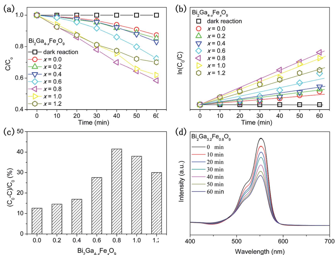
Fig. 4 (a) Photocatalytic degradation of RhB using \text{Bi}_2\text{Ga}_{4-x}\text{Fe}_x\text{O}_9 solid solutions under visible light irradiation. (b) First-order kinetic constants for the degradation of RhB under visible light irradiation. (c) The conversion efficiency of RhB over the solid solutions under visible light irradiation. (d) The UV-Vis absorption spectra of RhB at different concentrations using \text{Bi}_2\text{Ga}_{3.2}\text{Fe}_{0.8}\text{O}_9 as the photocatalyst under visible light irradiation. Photocatalytic conditions: 100 mg photocatalyst, 250 mL solution, RhB 20 ppm, pH = 6, V(\text{H}_2\text{O}_2) = 0.5 \text{ mL} , 300 W long-arc xenon lamp.
