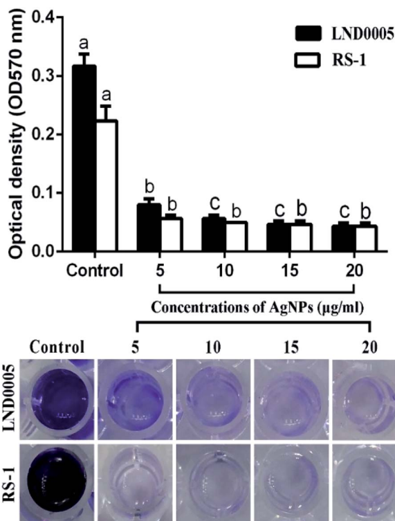
Fig. 6 Effect of the biosynthesized AgNPs on biofilm formation of Xoo strain LND0005 and Ao strain RS-1.
