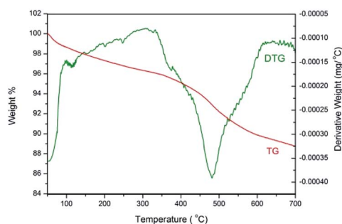
Fig. 7 Thermogravimetric (TG) and derivative thermogravimetric (DTG) curves for \text{NH-Cu(II)@MNP} .
