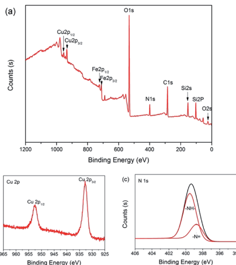
Fig. 6 The XPS spectra of the \text{NH-Cu(II)@MNP} catalyst 3 . (a) Survey scan; (b) Cu 2p and (c) N 1s.
