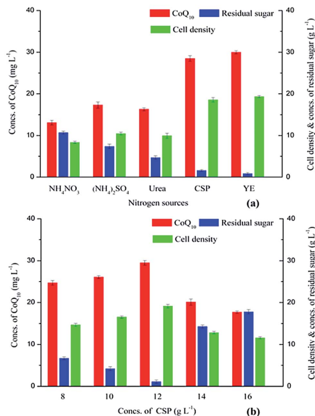
Fig. 2 Effects of different nitrogen sources on CoQ 10 titer, residual sugar and cell density (a) and the optimization of CSP concentration (b). All experiments were carried out at 30.00 ^{\circ} C and 220.00 rpm for 96.00 h on a rotary shaker, the pH was maintained at 7.00 and 250.00 mL flasks with a working volume of 100.00 mL were used.
