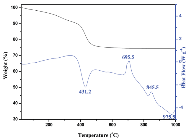
Fig. 2 TG-DSC curves of the prepared MBH sample.
