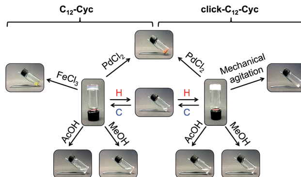
Fig. 5 Representative stimuli responsive map of organogels made of \text{C}_{12}\text{-Cyc} and \text{click-C}_{12}\text{-Cyc} in cyclohexane ( c = 15 \text{ g L}^{-1} ). Abbreviation: H = heating; C = cooling. [\text{AcOH}] = 1 \text{ M} .
