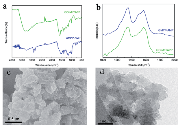
Fig. 1 (a) FT-IR spectra and (b) Raman spectra of GO-MnTAPP and GMPP@AMP; (c) SEM and (d) TEM of GMPP@AMP.
