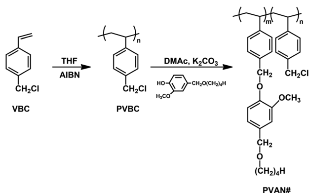
Fig. 1 Synthetic route to vanillin derivatives-substituted polystyrene (PVAN#), where # indicates the substitution ratio of vanillyl butyl ether containing monomeric units in the polymer.
