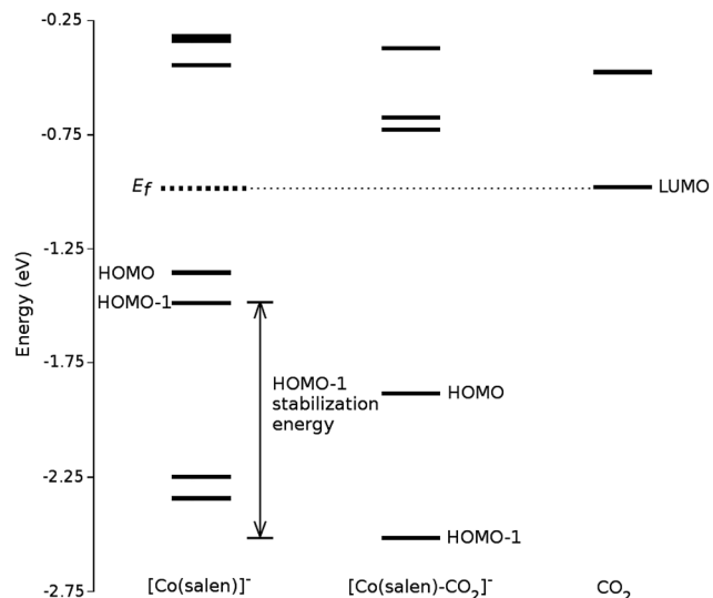
Fig. 8 Molecular orbital diagram of [Co(salen)] - , [Co(salen)-CO 2 ] - , and CO 2 . The figure shows the alignment of CO 2 LUMO with the Fermi energy of [Co(salen)] - , explaining the possibility of back-donation and charge transfer.
