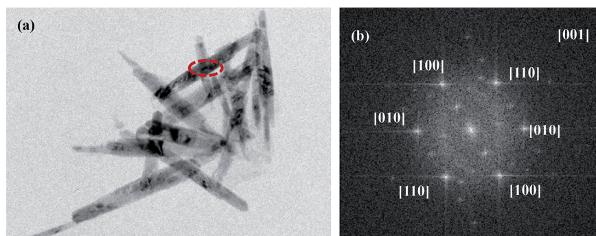
Fig. 5 TEM images (a) and SAED patterns (b) of \text{Fe}_2\text{O}_3/\text{rGO} .
