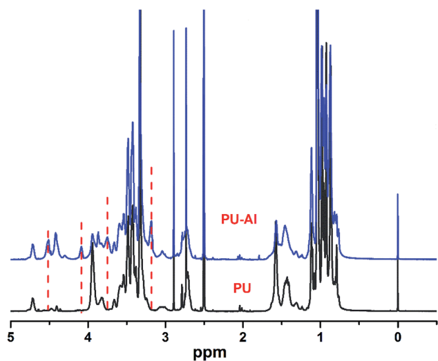
Fig. 4 1 H NMR spectra of non-clickable polyurethane (PU), clickable polyurethane with side-chain alkyne (PU-AI).
