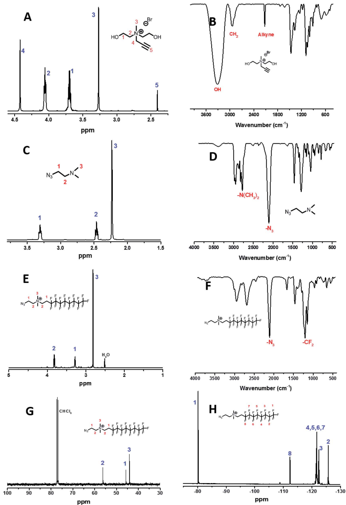
Fig. 2 1 H NMR and FT-IR spectra of M1 (A and B), M2 (C and D), M3 (E and F) and 13 C/ 19 F NMR spectra of M3 (G and H).
