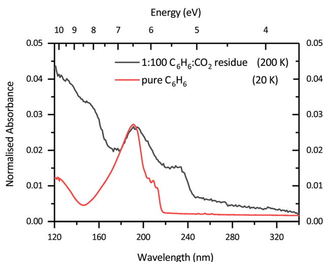
Fig. 4 VUV photoabsorption spectra of a 1 : 100 C_6H_6 : CO_2 mixture which was irradiated with 1 keV electrons for 180 min and annealed to 200 K (black) to form a residue compared with pure benzene (red) at 20 K. The pure benzene spectrum at 20 K has been normalised to the peak height at \lambda = 190 nm of the 1 : 100 C_6H_6 : CO_2 residue.
