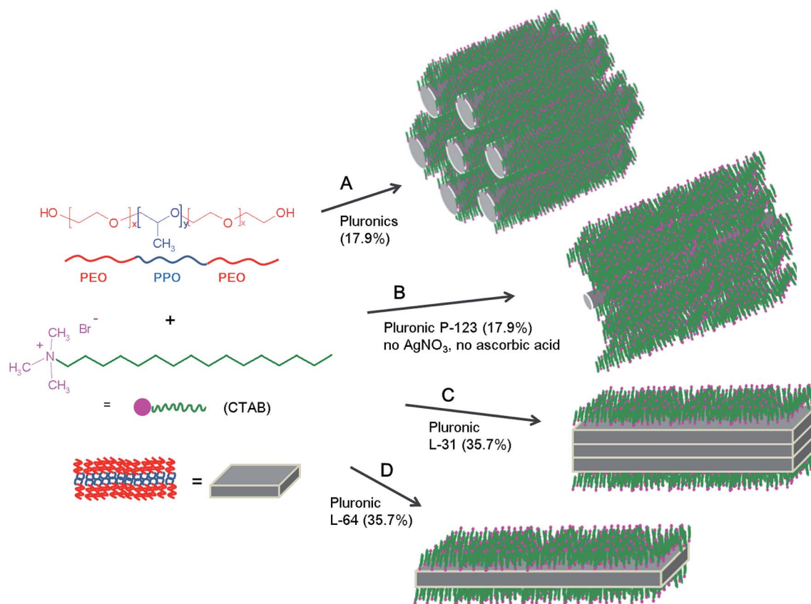
Scheme 1 The process for the formation of macroscale rods and plates from the surfactant mixture of CTAB and Pluronics in the presence (A, C and D) and in the absence (B) of AgNO 3 and ascorbic acid.
