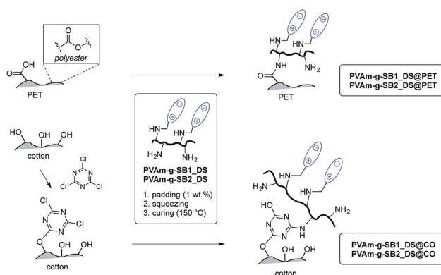
Scheme 2 Finishing of polyester (PET) and cotton (CO) with sulfobetaine-modified PVAm. Whereas PVAm can be covalently linked to PET directly by heating, a triazine-based anchor was used for cotton fabrics. The DS of the polymers varied from 20–80%.
