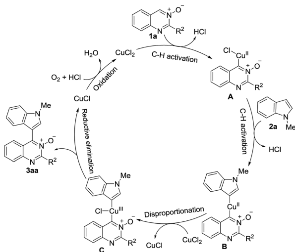
Scheme 4 Plausible mechanism.
