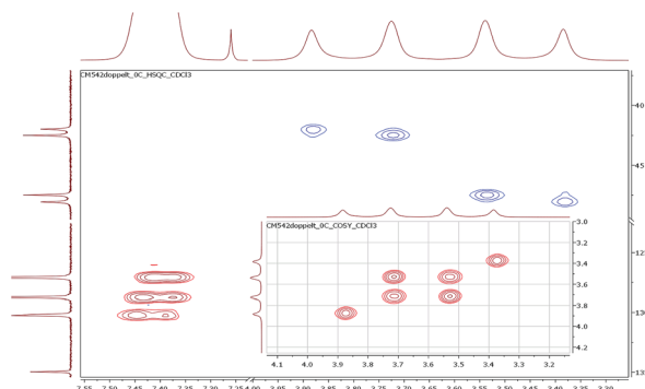
Fig. 2 Part of the ^1\text{H} , ^{13}\text{C} -HSQC and H,H-COSY (inset) spectra using the symmetrically disubstituted compound 4a at 0 °C.
