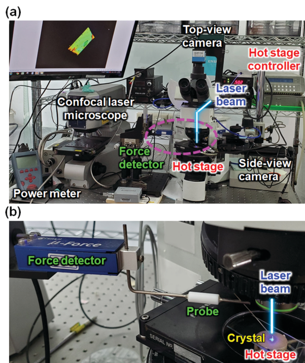
Fig. 14 Photographs of the setup for the photoirradiation experiments. (a) Overall view and (b) expanded view around the crystal sample. A laser beam line is illustrated.
