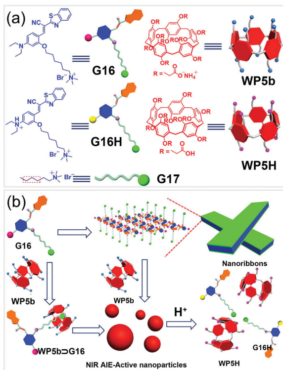
Fig. 20 (a) Chemical structures of the guests, WP5b , and WP5H , and (b) schematic illustration of self-assemblies of G16 and WP5b \supset G16 and pH responsiveness of the NPs. Reproduced with permission from ref. 117. Copyright 2016, American Chemical Society.
