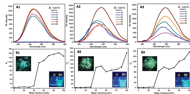
Fig. 3 Fluorescent spectra of TPE-L-Glu, cis -TPE-L-DGlu and trans -TPE-L-DGlu in THF/water mixed solvents with different f_w (A1–A3); plot of I_0/I_w values versus f_w (B1–B3), where I_0 represents the emission intensity in THF. Concentration: 1 \times 10^{-5} M; excitation wavelength: 340 nm. Inset: Photographs of TPE-L-Glu, cis -TPE-L-DGlu and trans -TPE-L-DGlu in solid and THF/water mixtures with 0 and 99% f_w under 365 nm UV lamp.
