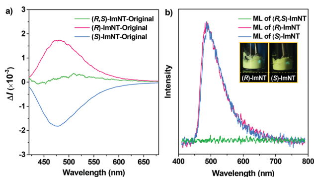
Fig. 3 CPL (a) and ML spectra (b) of the as-prepared samples of (R,S)-ImNT, (R)-ImNT and (S)-ImNT under ambient conditions. The insets in (b) depict the ML images of (R)-ImNT and (S)-ImNT in daylight.
