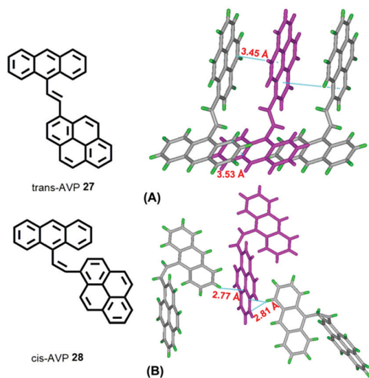
Fig. 18 Structures of (A) trans -AVP 27 and (B) cis -AVP 28, and their crystal packing.
