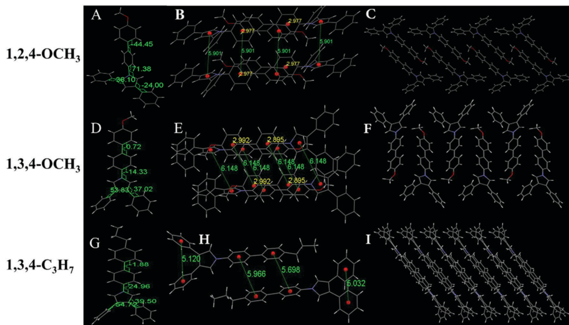
Fig. 3 (A) Molecule structure, (B) interaction distance of the \pi \cdots \pi and C-H \cdots \pi interactions and (C) stacking image along the b -axis of 1,2,4-OCH 3 . (D) Molecule structure, (E) interaction distance of the \pi \cdots \pi and C-H \cdots \pi interactions and (F) stacking image along the b -axis of 1,3,4-OCH 3 . (G) Molecule structure, (H) interaction distance of the \pi \cdots \pi and C-H \cdots \pi interactions and (I) stacking image along the b -axis of 1,3,4-C 3 H 7 . Gray color corresponds to carbon, white to hydrogen, red to oxygen and blue to nitrogen.
