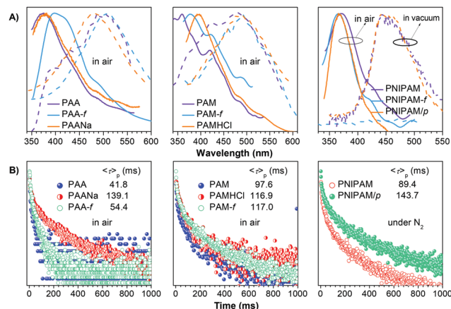
Fig. 4 (A) Emission spectra with \tau_0 of 0 (solid line) and 0.1 ms (dash line) and (B) RTP decay curves of different films ( f ) and powders in air, under nitrogen, or in vacuum. Detailed \lambda_{ex} s for the emission measurement and monitored wavelengths for the lifetime test are listed in Tables S1 and S2 (ESI † ).
