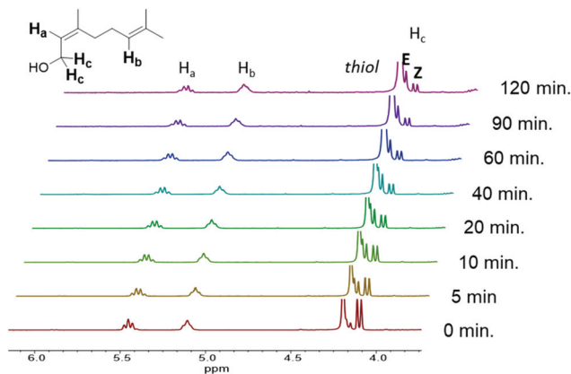
Fig. 3 1 H NMR spectrum of nerol prepolymer, with the terpene reacting with PETMP under irradiation at \lambda = 365 nm, displaying monomer isomerization over the course of 120 min.
