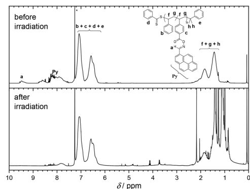
Fig. 2 ^1\text{H} NMR spectrum (400 MHz, \text{CDCl}_3 , 298 K) of CDB PS PyOHSty 1 before and after LED irradiation (430–435 nm). The magnetic resonance at 4.12 and 3.73 ppm originate by the fragmentation of the RAFT moiety upon light exposure. The magnetic resonance marked with an asterisk is assigned to \text{CHCl}_3 .
