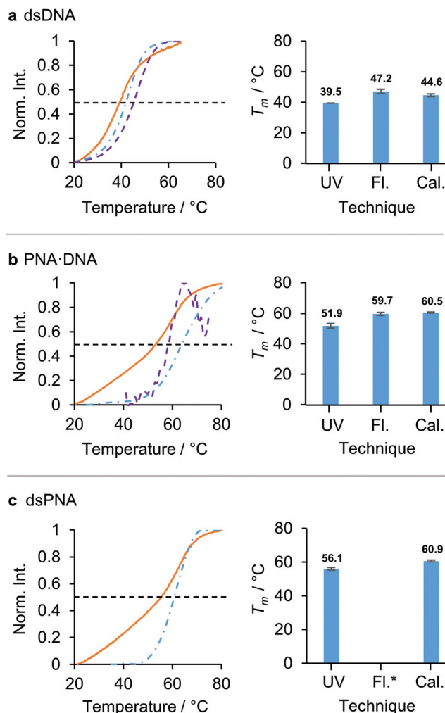
Fig. 1 Comparison of three techniques for the measurement of the T_m of nucleic acid duplexes in aqueous solution: UV absorbance (UV, orange solid line), fluorescence (FI., violet dashed line) and calorimetry (Cal., blue dashed-dotted line). The black dashed line indicates the 50% maximum intensity from which the T_m s were calculated. The duplexes studied were: (a) dsDNA, (b) PNA-DNA, (c) dsPNA. The calculated melting temperatures for each duplex are displayed in the bar charts in the right hand column. *Fluorescence was not measurable. The normalised intensities (norm. int.) corresponded to: UV absorbance at 260 nm, fluorescence emission measured in counts and the numeric integral of the excess heat capacity. (dsDNA was excited at 495 nm and the fluorescence emission was measured at 512 nm. PNA-DNA was excited at 290 nm and the fluorescence emission was measured at 340 nm. Sigmoidal baselines were fitted and subtracted to produce the molar excess heat calorimetry signals. 26 Sequences: [10]-DNA/PNA1 5'/N – TCA CTA GAT G – C/3' [10]-DNA/PNA2 5'/N – CAT CTA GTG A – C/3'. For full sequences and modifications, see section 1 ESI.† For solvents, concentrations and heating rates see Table S3 ESI.†)
