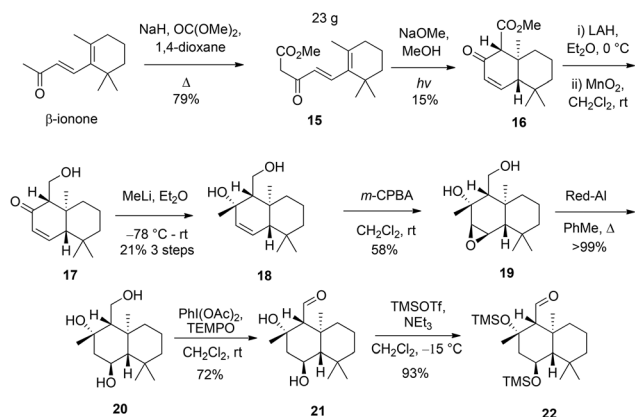
Scheme 3 Synthesis of drimane aldehyde 21 .
