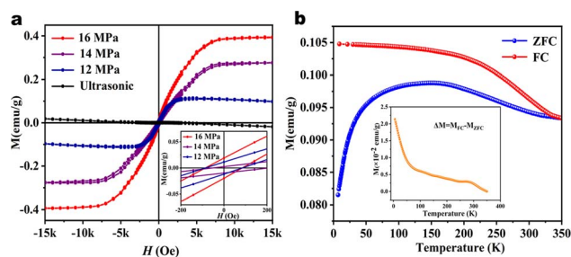
Fig. 5 (a) M – H curves of B-GO-X MPa and ultrasonicated graphite at 300 K. (Inset): M – H curves near H = 0 Oe. (b) FC-ZFC magnetization curves of B-GO-16 MPa at an external magnetic field of 500 Oe. (Inset): \Delta M = M_{FC} - M_{ZFC} curve of B-GO-16 MPa.
