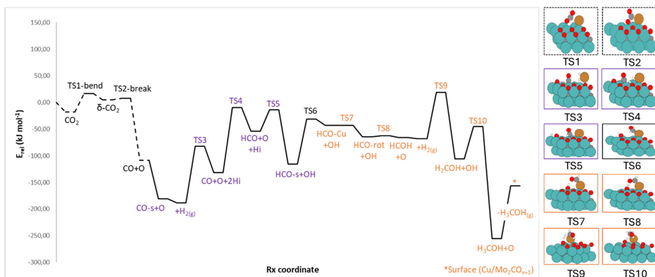
Fig. 5 Energy profile for the reaction of CO 2 and 2H 2 to form methanol from HCOH* species on the support (purple labels) to HCOH* species on the Cu center (orange labels). The dashed line shows steps that are common for all profiles. Energies of minima and transition states (framed) are referenced against the sum of the initial reactants and catalyst energies in kJ mol -1 ( E_{rel} ).
