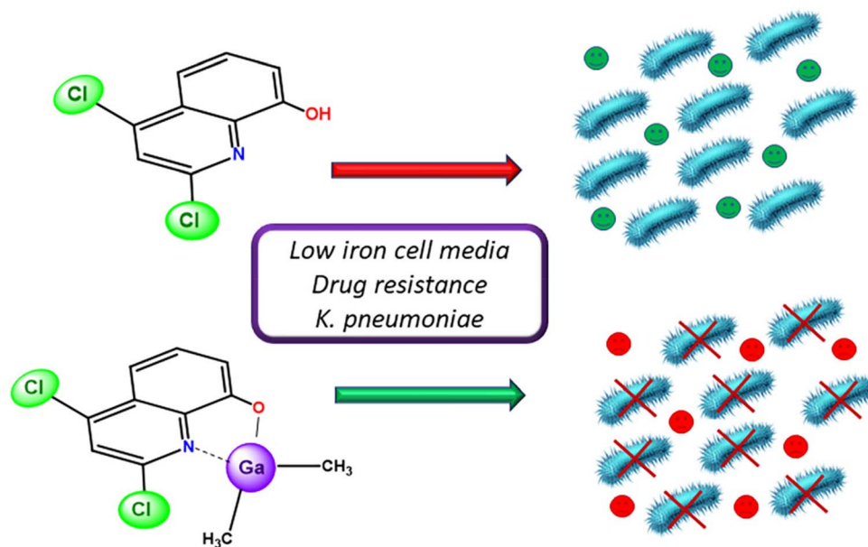
Fig. 3 The enhanced anti-bacterial activity of four dimethyl gallium 8-quinolinol complexes was determined in physiologically relevant low-iron media. Exceptional activity was observed toward a multi-drug resistance strain of the ESKAPE pathogen K. pneumoniae . Protein-uptake studies suggest the methyl substituted complexes do not undergo rapid uptake or exchange with iron-binding proteins. 23
