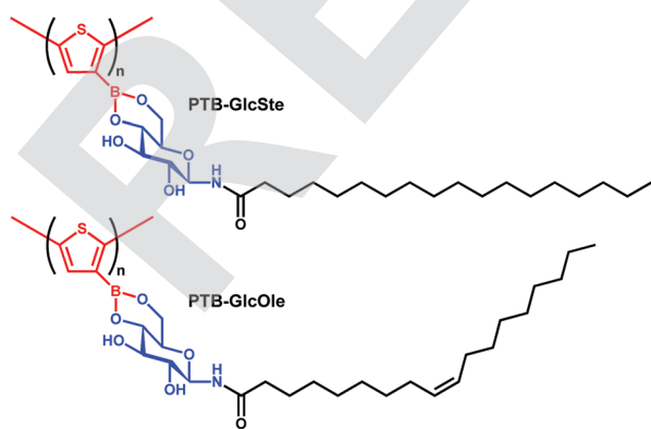
Scheme 1 Chemical structures of PTB-GlcSte and PTB-GlcOle polymers.
